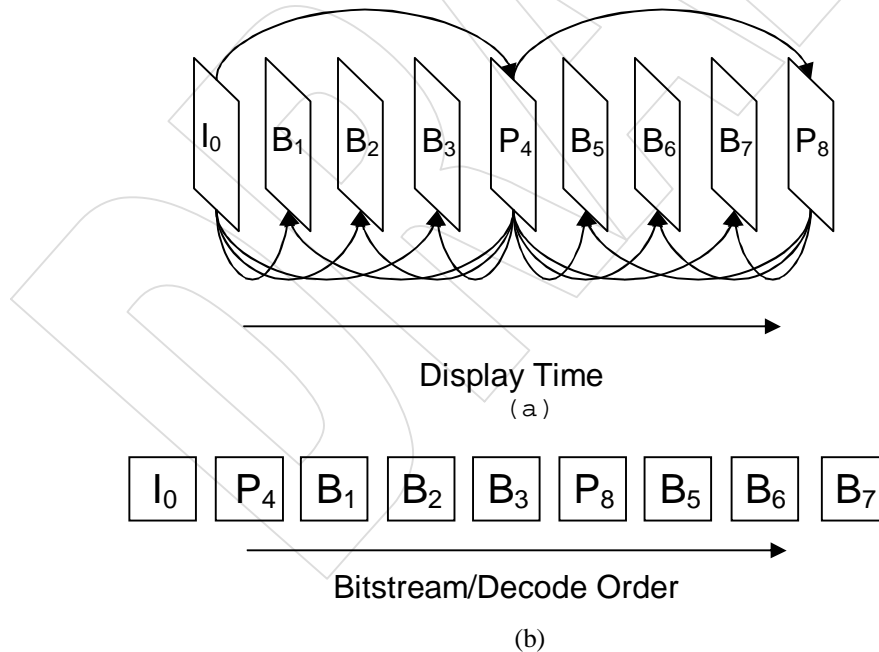
Figure 4.2: (a) Display Order. (b) Bitstream and Decode Order
