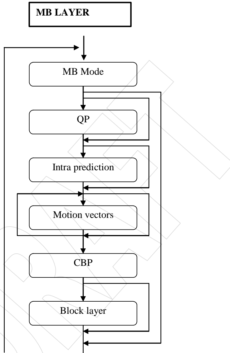
Figure 2 Macroblock Layer
