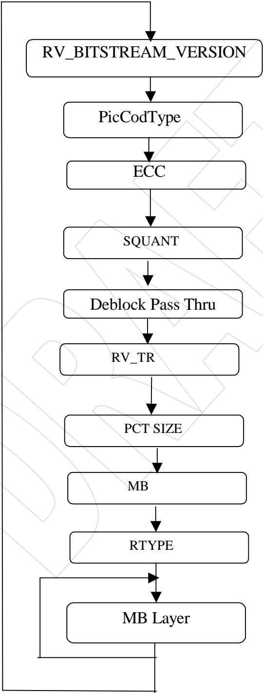
Figure 5.1 Slice Layer
